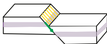
faille normale
