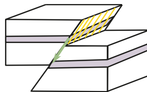
faille inverse
