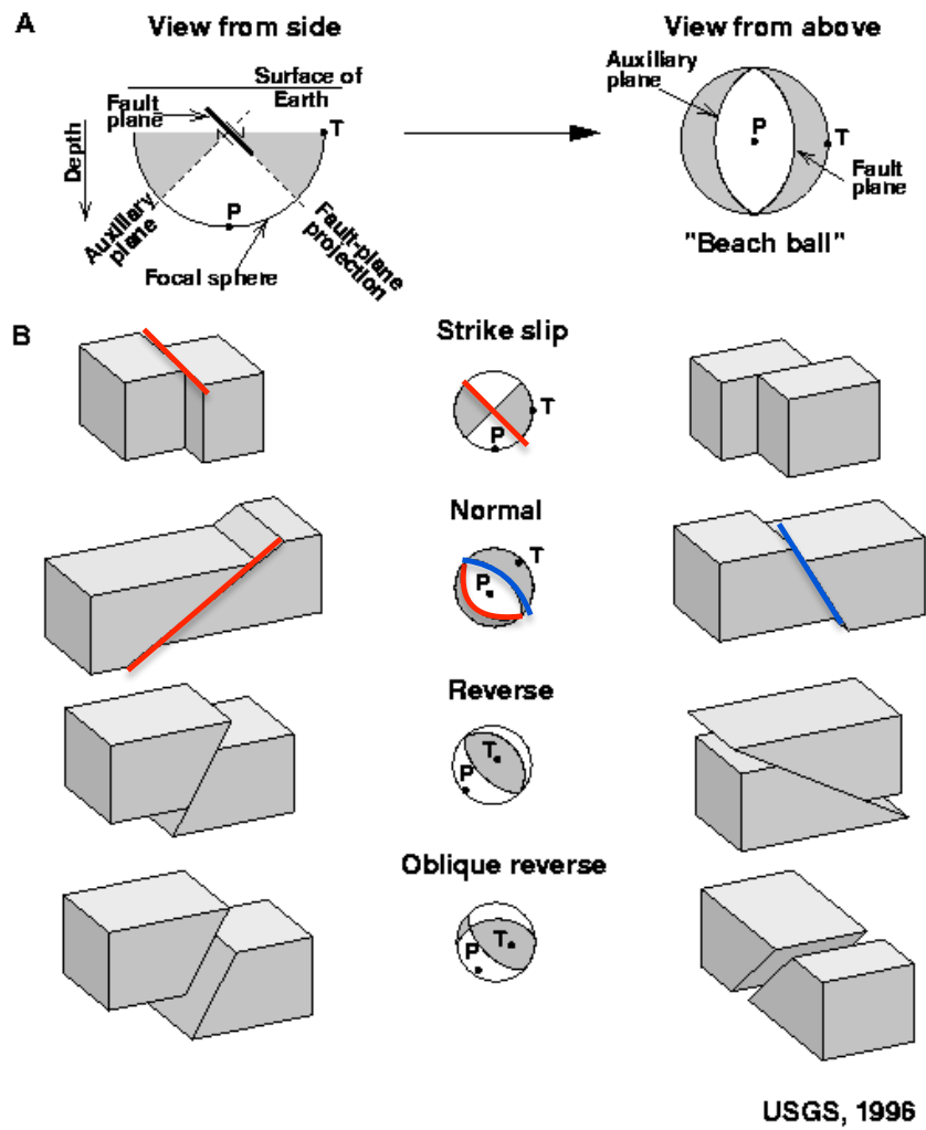
Figure 6 : hodochrones (in Renart et al., 2016)
